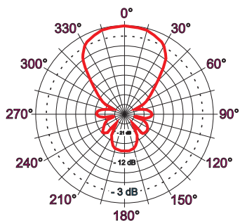
GSM (890-960 MHz)
