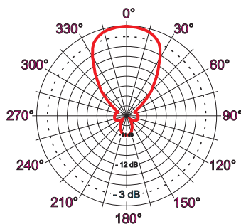
DCS (1710-1880 MHz)
